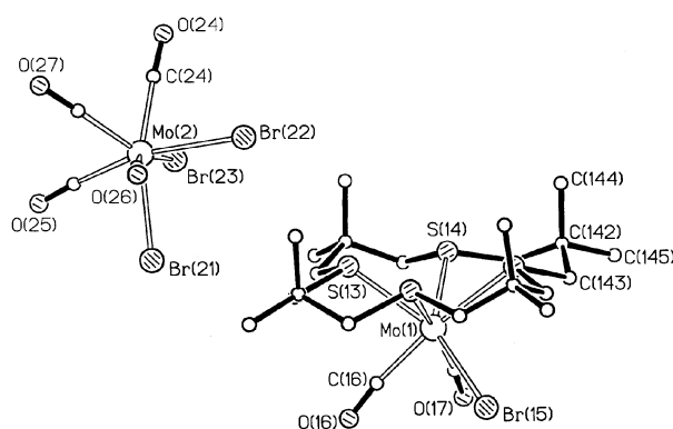
Fig. 1 Structure of [MoBr(CO) 2 (Me 8 [16]aneS 4 )] [MoBr 3 (CO) 4 ] 1 . The minor component of the bromide ligand and the atoms of the unresolved solvent molecule(s) are not shown
