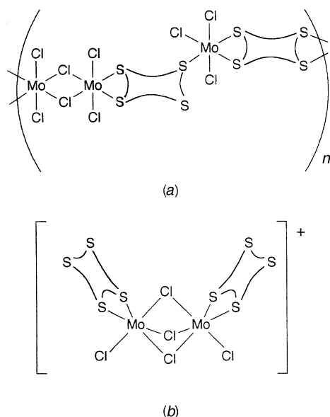
Fig. 6 Proposed structures of [\{\text{Mo}_3\text{Cl}_9(\text{[16]aneS}_4)_2\}_n] 7 (a) and [\text{Mo}_2\text{Cl}_5(\text{[16]aneS}_4)_2]^+ 8 (b)
