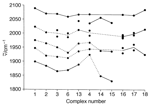
Fig. 3 Infrared data for the ionic complexes in the carbonyl region. Complex numbers are as in Table 1; additional data for [\text{MI}(\text{CO})_3\text{([9]aneS}_3)]^+ ( \text{M} = \text{Mo} 14 or \text{W} 15 ), 24 [\text{MI}_3(\text{CO})_4]^- ( \text{M} = \text{W} 16 or \text{Mo} 17 ) 23 and [\text{WBr}_3(\text{CO})_4]^- 18 18 were taken from the literature. Solid and broken lines indicate probable and possible correlations respectively
