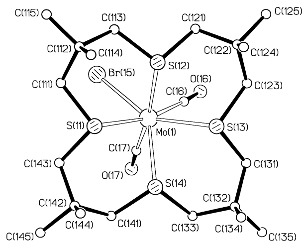
Fig. 2 The cation of complex 1 , showing the atom numbering scheme of the macrocyclic ligand, common also to that in 3 and 4
