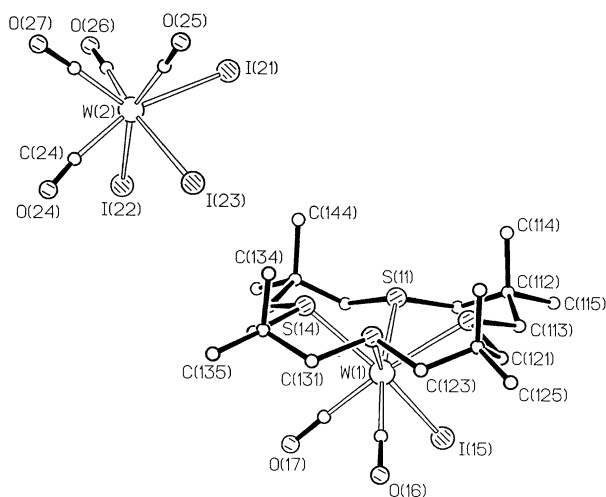
Fig. 4 Structure of [\text{W}(\text{CO})_2(\text{Me}_8[16]\text{aneS}_4)][\text{W}(\text{CO})_4] \mathbf{3}
