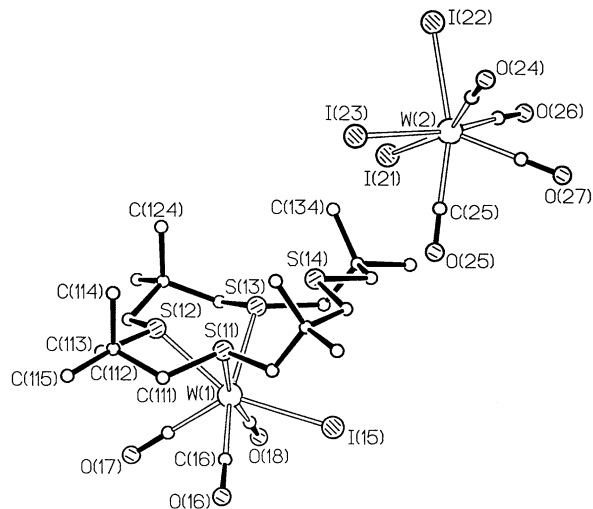
Fig. 5 Structure of [\text{W}(\text{CO})_3(\text{Me}_8[16]\text{aneS}_4)][\text{W}(\text{CO})_4] \mathbf{4}
